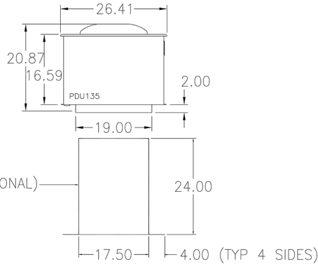
FAN AND ROOF CURB DIMENSIONS
