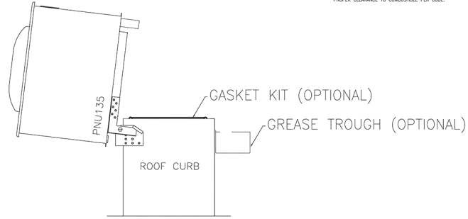
FAN AND HINGE KIT IN OPEN POSITION DETAIL
