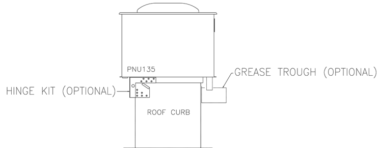
FAN AND HINGE KIT IN CLOSED POSITION DETAIL
