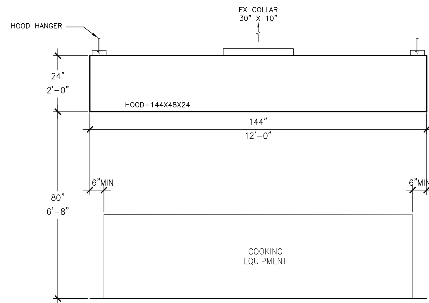
FRONT VIEW 1/2" = 1'-0"
